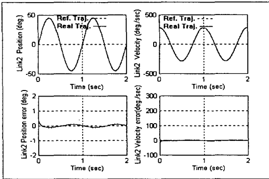
Fig. 4 Simulation results of position and velocity trajectory tracking for link 2.(2 kg payload)
