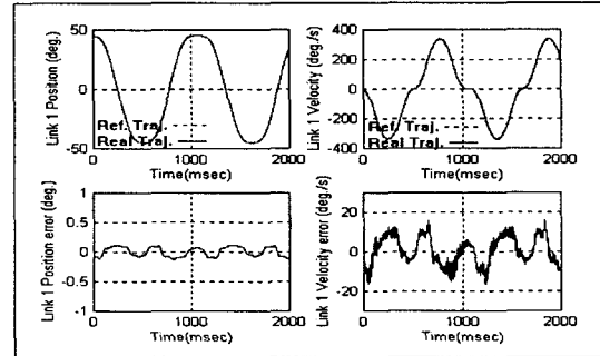
Fig. 6 The experimental results of SOFC for position and velocity trajectory tracking of link 1.(2.0kg payload)
