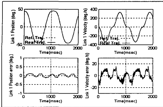
Fig. 9 The experimental results of PID controller for position and velocity trajectory tracking of link 6. (2.0kg payload)
