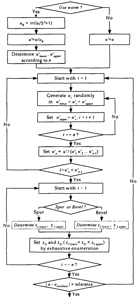
Fig. 1 Flow chart of random search method for cylindrical, bevel and worm gears
