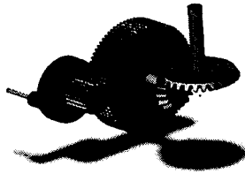
Fig. 3 Mechanism H-S-B(helical-spur-bevel) in three stages
