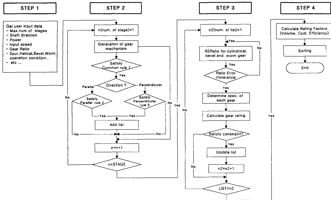
Fig. 2 Generation and preliminary design algorithm of compound multi-stage drive mechanisms
