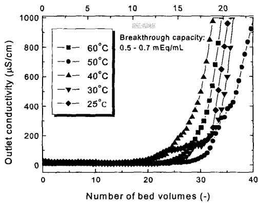
Fig.3 Dynamic capacity measurements for Zn(II) adsorption onto mixed resin of IRN150 at various temperature.
