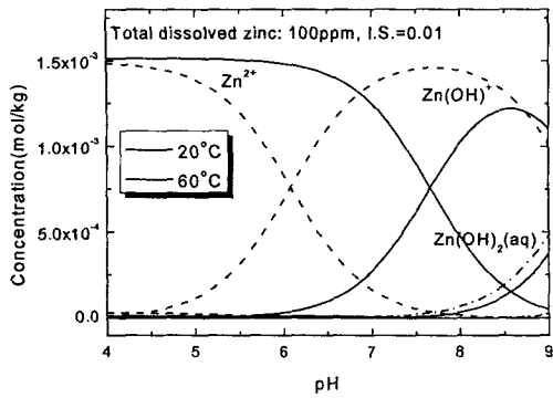
Fig.1 Aqueous equilibrium distribution of dissolved zinc species at different pH (20°C and 60°C).
