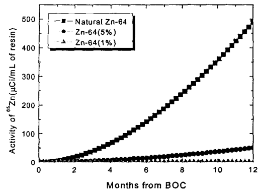
Fig.4 Projected activity of ^{65}Zn on the mixed bed demineralizer resin for the addition of natural and depleted zinc.
