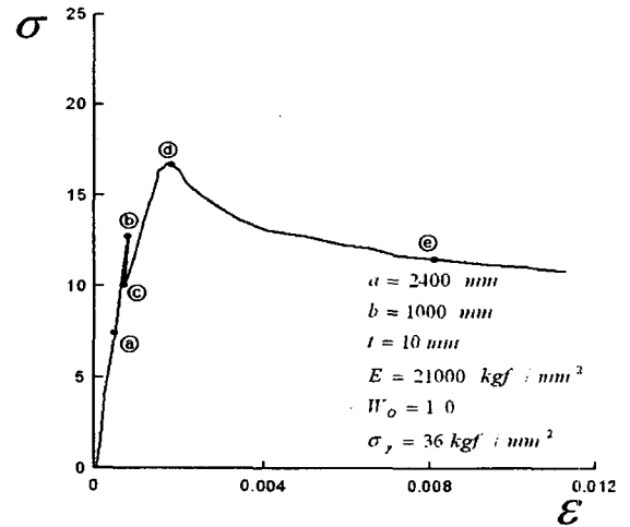
Fig. 6 A comparison stress with strain curve under thrust (a/b=2.4)
