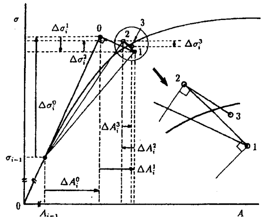
Fig. 1 Arc-length approach with full newton-raphson method
