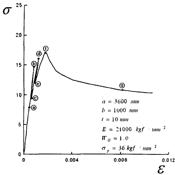
Fig. 8 A comparison stress with strain curve under thrust (a/b=4.4)
