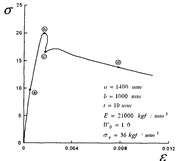
Fig. 4 A comparison stress with strain curve under thrust (a/b=1.4)
