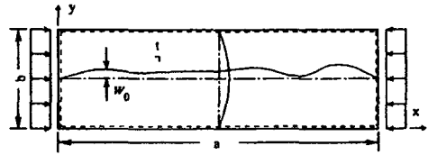
Fig. 2 Rectangular plate with initial deflection under thrust
