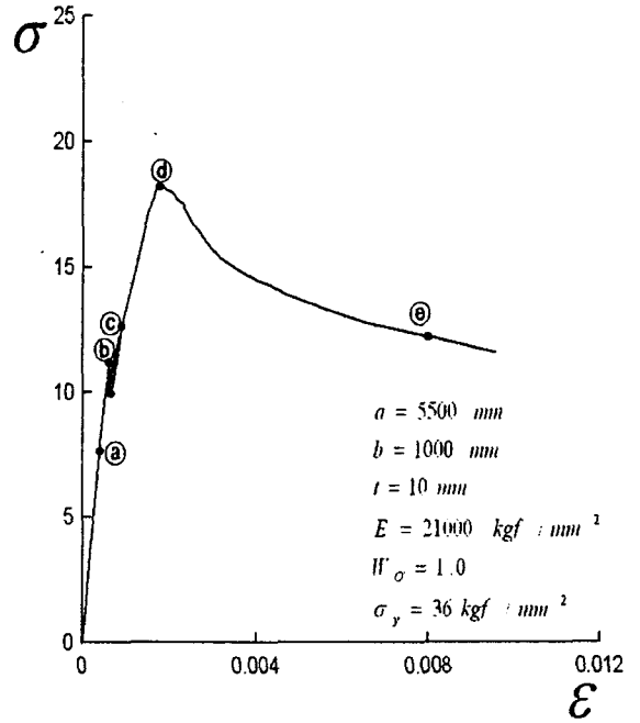
Fig. 9 A comparison stress with strain curve under thrust (a/b=5.5)
