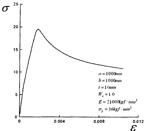
Fig. 3 A comparison stress with strain under thrust (a/b=1.0)
