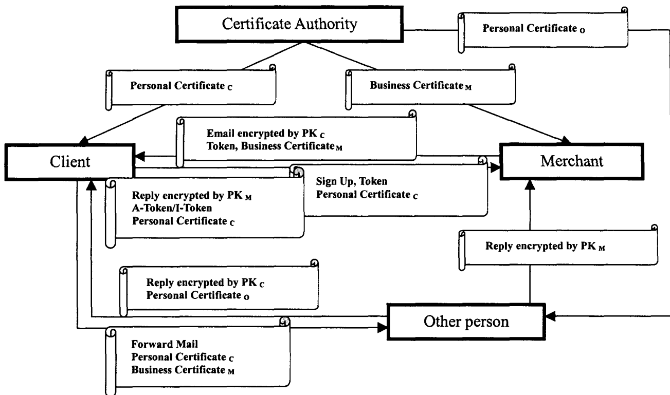
Figure 4 - Architecture of Business to Customer with Token
