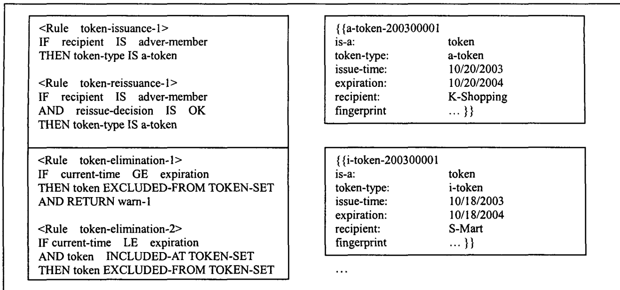
Figure 2 - Illustrative Token Management Rules and Knowledge Base
