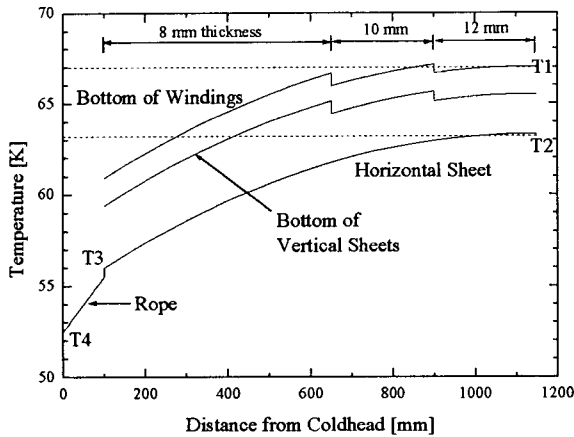
Fig. 5. Temperature distributions from coldhead to HTS windings ( Q_{ac}=150 W)
