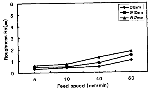
Fig. 7 Roughness of Surface for inside hole drilled by drill diameters (Cutting speed : 47.1m/min)
