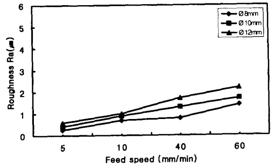
Fig. 6 Roughness of surface for inside hole drilled by drill diameters (Cutting speed : 25.12m/min)
