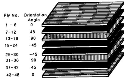
Fig. 1 Stacking sequences method of multi-direction hand lay-up
