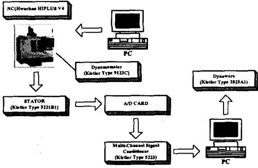
Fig.3 Schematic diagram of experimental measuring system
