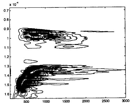
Figure 3 Contour plot of the wavelet transform of Lamb wave signal
