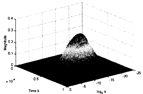
Figure 2 3-D plot of the wavelet transform of Lamb wave signal
