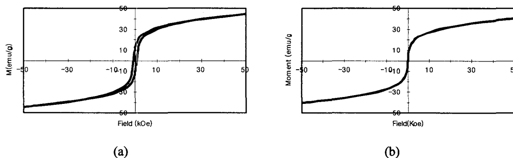
Fig.1. Magnetization curves of Zn-ferrite particles at (a) 5 K, (b) 100 K.
