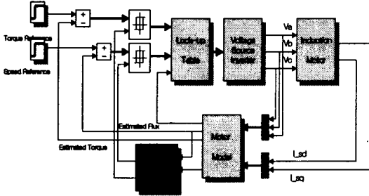
Fig. 3 Online Hysteresis Band Amplitude Calculator of DTC
