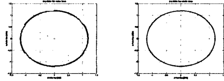
Fig. 9 Stator Flux Vector Locus for \Delta\lambda=0.0073 (Wb) \Delta T=0.6322 (Nm) and Proposed strategy
