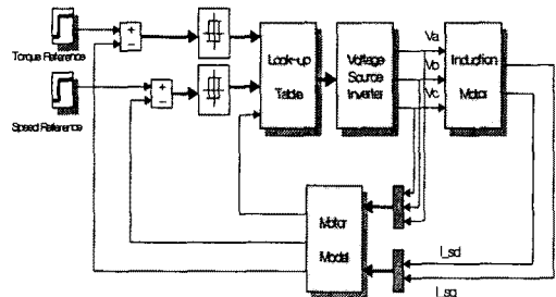
Fig. 1 Basic scheme of Conventional Direct Torque Control Strategy
