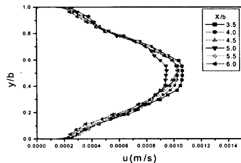
Fig. 4 Velocity Distributions along the Test Tube for Re=2.267 without D.C Voltage.
