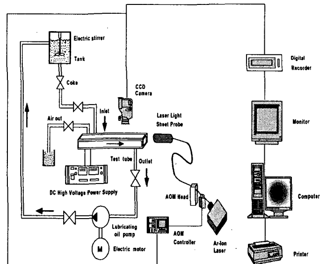
Fig. 1 Experimental Apparatus and PIV System
