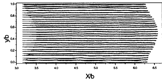
Fig. 3 Velocity Vectors Distributions along the Test Tube for Re=2.267 without D.C Voltage.
