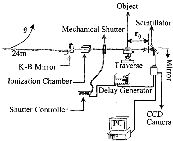
Fig. 1 Schematics of synchrotron X-ray micro imaging system
