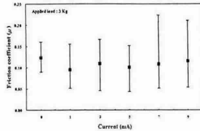
Fig. 6 Effect of current on friction coefficient for 3kg
