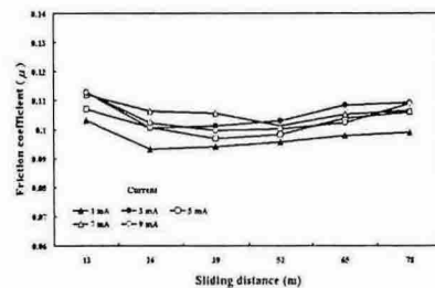
Fig. 11 Relation between sliding distance and friction coefficient for 7 kg
