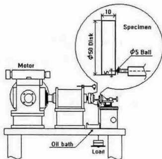
Fig 1. Schematic diagram of ball on disk type tester
