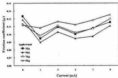
Fig. 8 Relation between of current and friction coefficient
