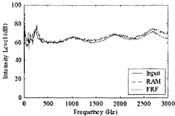
Fig.5 Comparison of input power with in-plane vibration intensity at x=0.6\text{m} on a beam.
