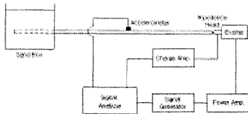
Fig. 2 Overview of the system setup
