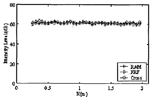
Fig.4 In-plane vibration intensity of a beam at 1500 Hz.
