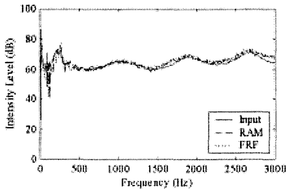
Fig.6 Comparison of input power with in-plane vibration intensity at x=1\text{m} on a beam.
