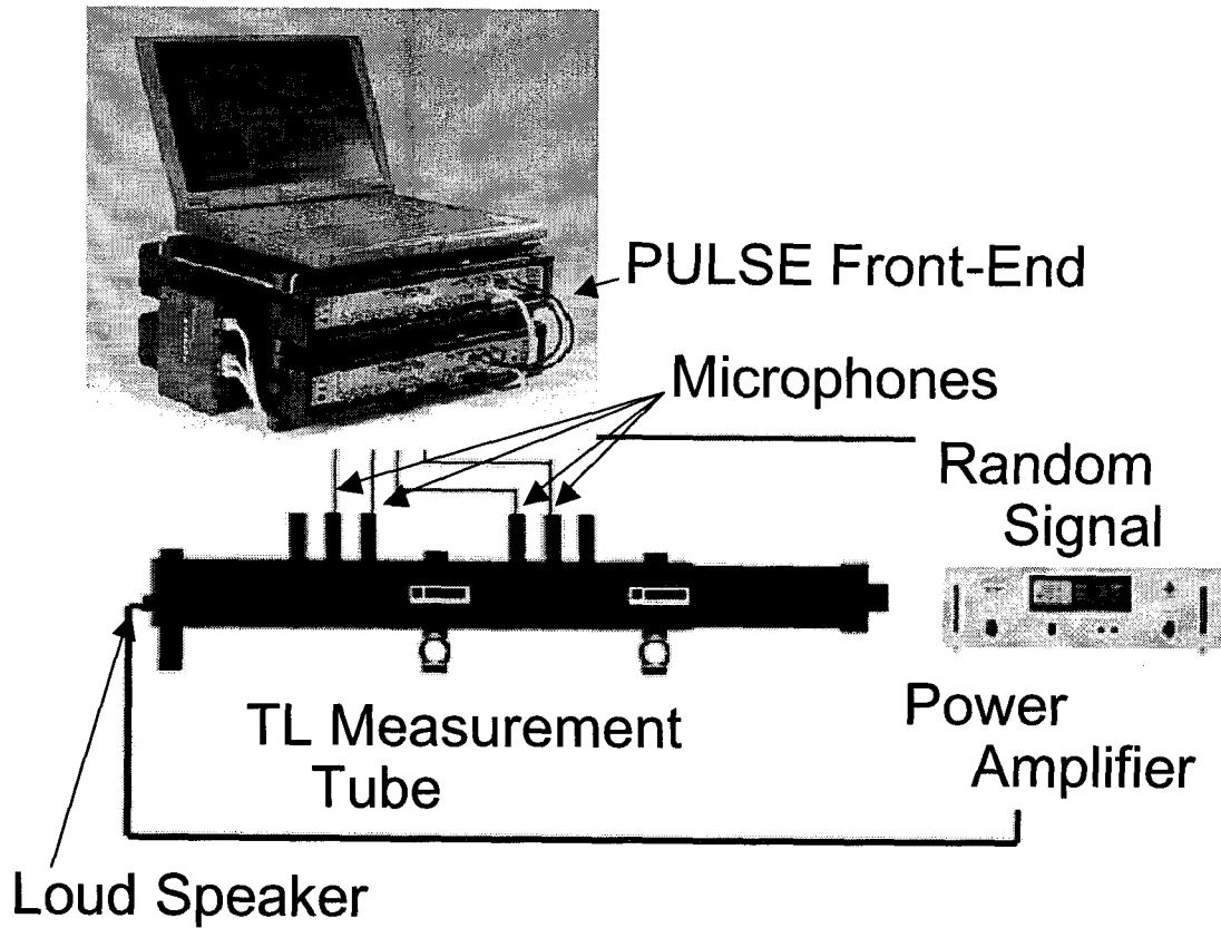
Fig. 2 System Configuration of Transmission Loss Measurement System
