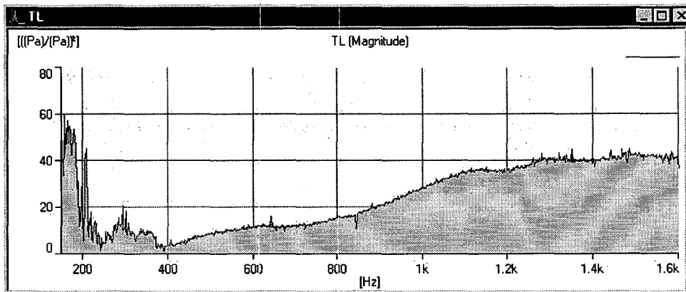
Fig. 5 Transmission Loss Coefficient
