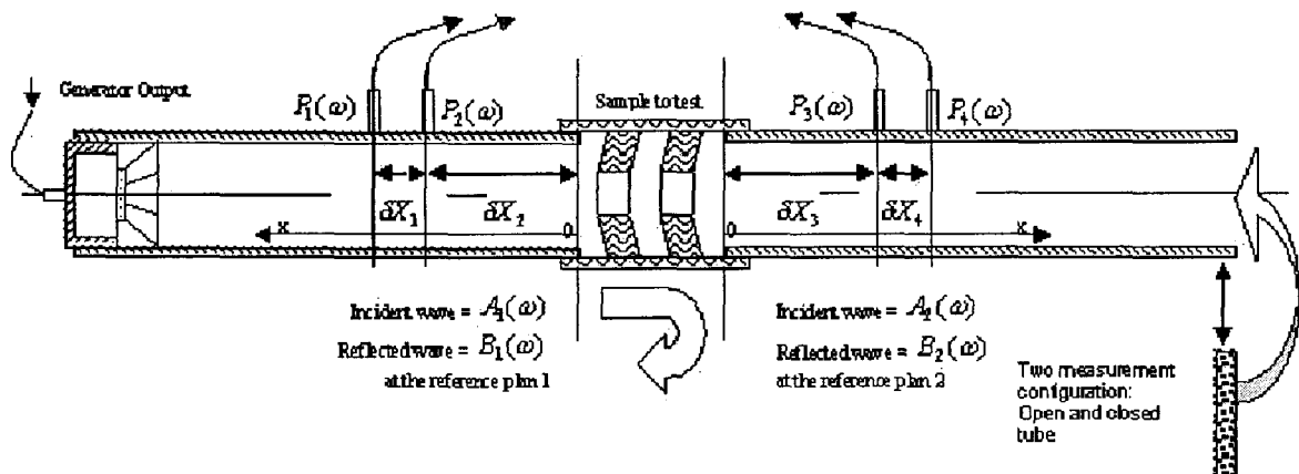
Fig. 1 Systemic Sketch of Incident & Reflecting Waves
