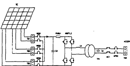
Fig. 3 Inverter configuration
