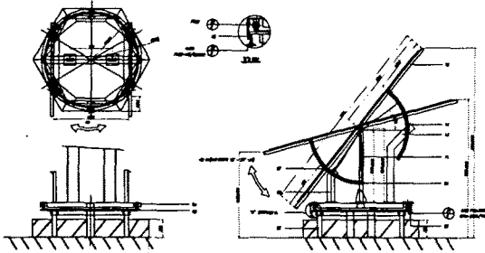
Fig. 2 Support equipment
