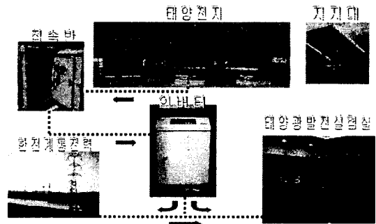
Fig. 1 3kW utility interactive residential photovoltaic generation system
