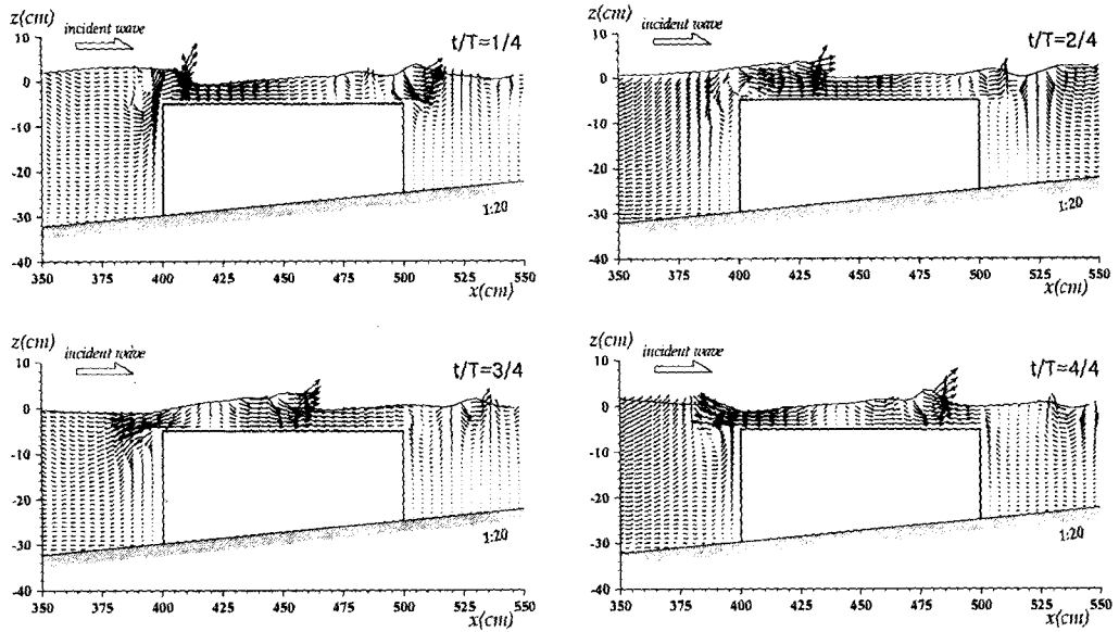
Fig. 3. Wave profile and velocity field in the vicinity of submerged breakwater for Case1.
