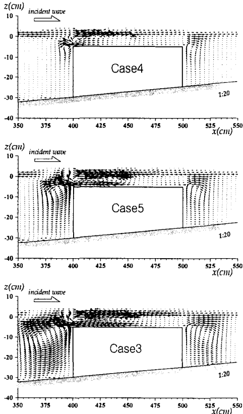
Fig. 7. Averaged-velocity fields for Case3, Case4 and Case5.
