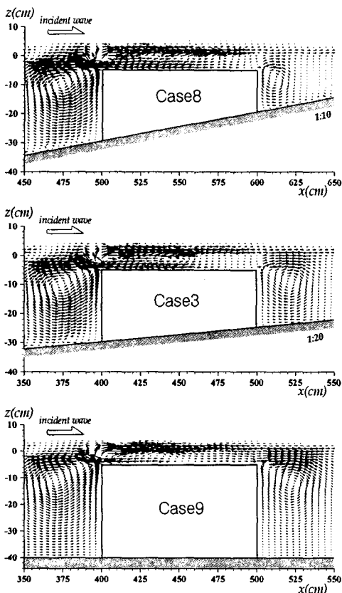
Fig. 9. Averaged-velocity fields for Case3, Case8, and Case9.
