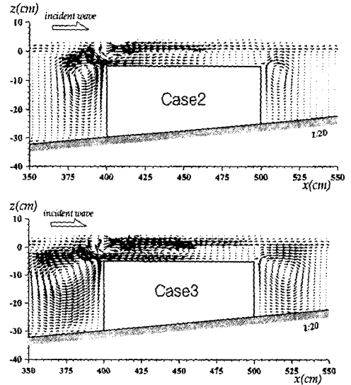
Fig. 6. Averaged-velocity fields for Case1 ~ Case3.
