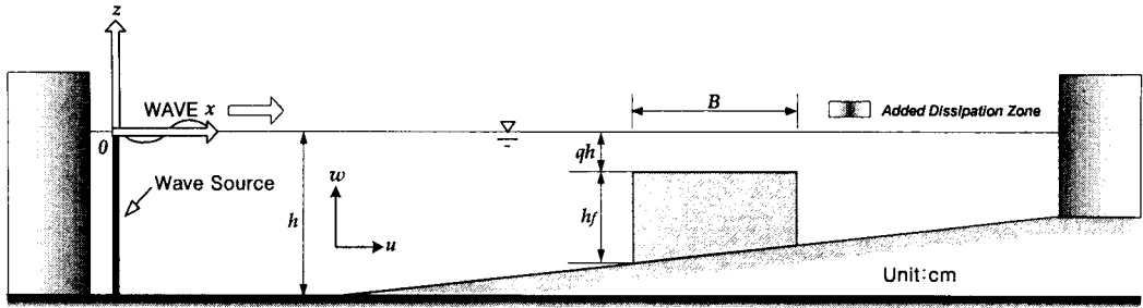
Fig. 1. Definition sketch of numerical wave channel.
