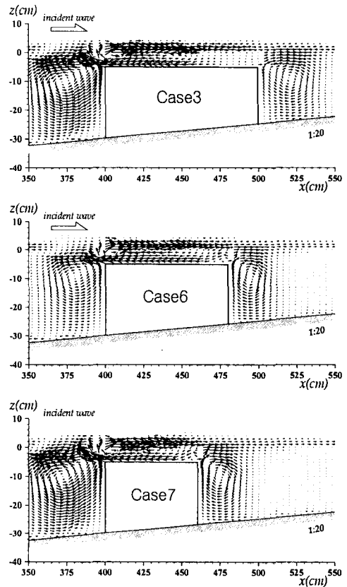
Fig. 8. Averaged-velocity fields for Case3, Case6, and Case7.
