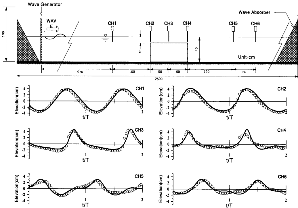
Fig. 2. Comparison of numerical solution results and experiment data (○: Experiment —: Numerical result).
