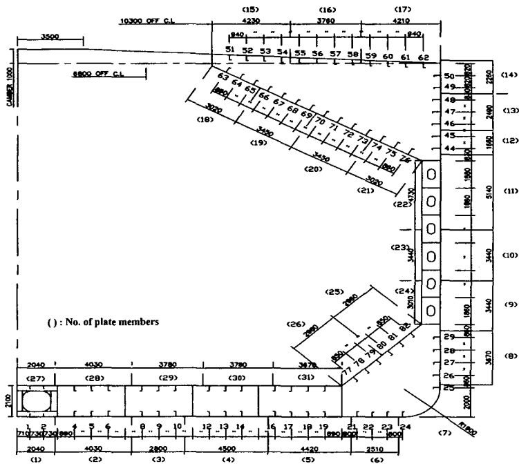
Fig. 2 Longitudinal members of double hull B/C (Type B)
