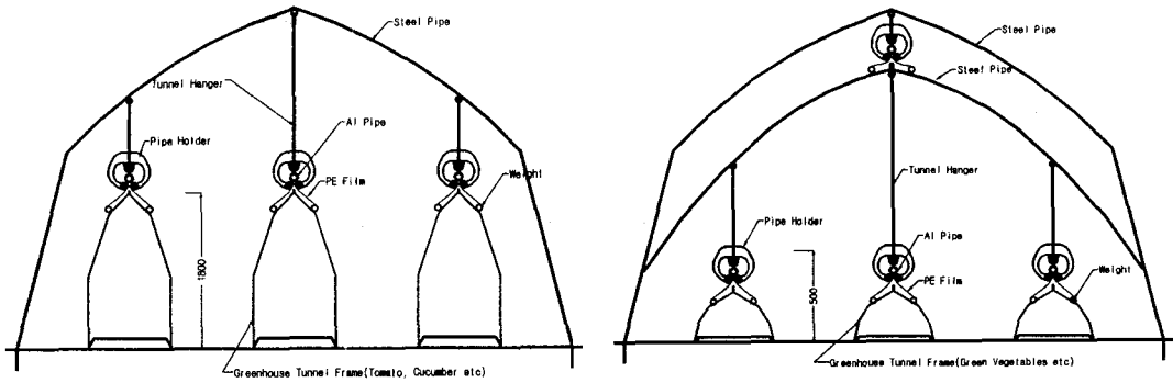
Fig. 1. Schematic diagram of opening & closing apparatus for thermal tunnel.
