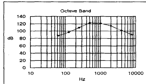
Fig. 4 Sound power level of curving-noise
