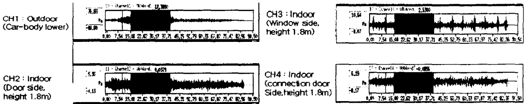
Fig. 6 4 channel time-series of curving noise
