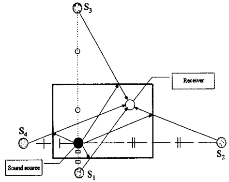
Fig. 2 First-order mirror image and reflection paths
