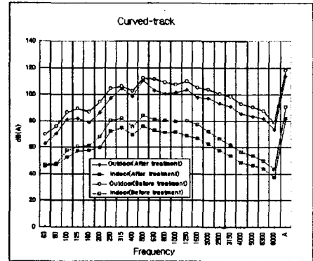
Fig. 9 Comparisons of measured sound pressure levels before and after treatment
