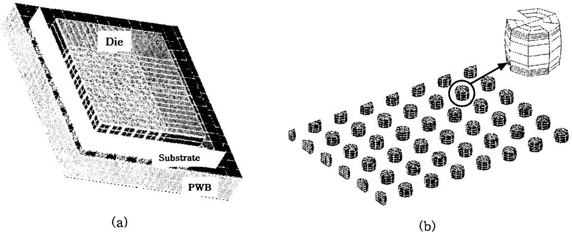
Fig. 1 3-D Finite element mesh model of FC-BGA on PWB (a) 165 FC-BGA (b) global solder ball
