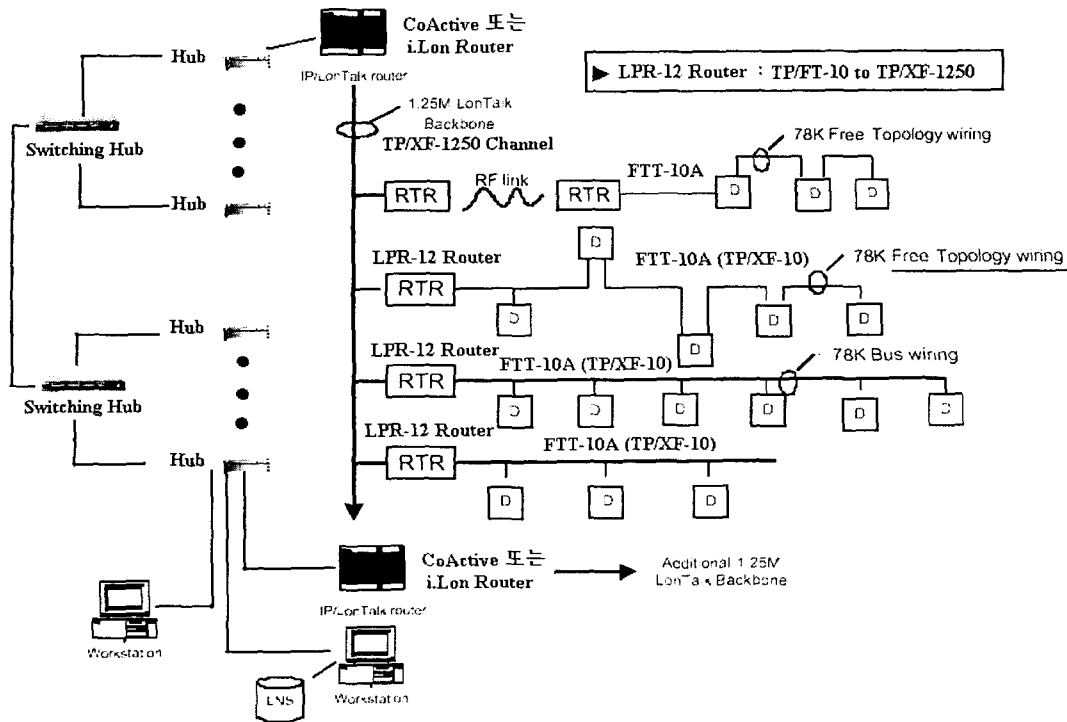
Fig. 6 Conceptual configuration of LonWorks network for distributed fire alarm systems
