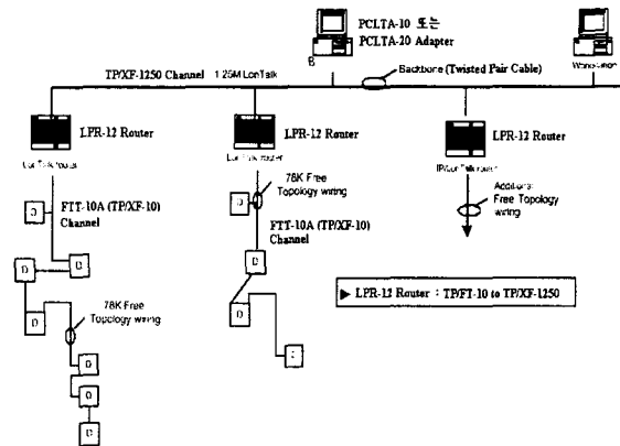
Fig. 4 A small scale configuration of LonWorks network fire alarm signaling system
