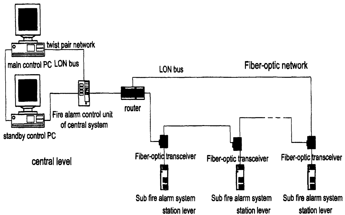
Fig. 5 An designed example of fire alarm system configuration
