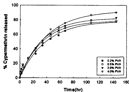
Fig. 3 Effect of PVA concentration on the release rate of cypermethrin from polyurea microcapsules.
