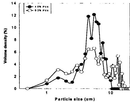
Fig. 1 Particle size distribution of polyurea microcapsules containing Cypermethrin from different PVA concentrations.
