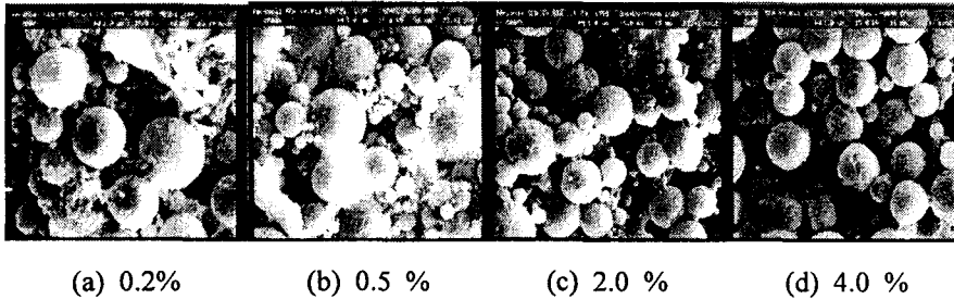
Fig. 2 SEM photographs of polyurea microcapsules containing cypermethrin from different PVA concentrations. (a) 0.2% , (b) 0.5% , (c) 2.0% , (d) 4.0%
