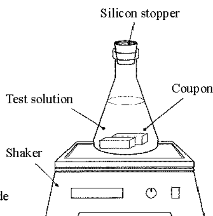
Fig.2 Apparatus of exposure experiment
