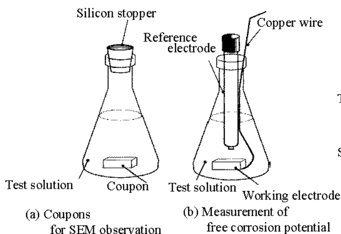
Fig.1 Experimental set up showing the details of coupon exposure
