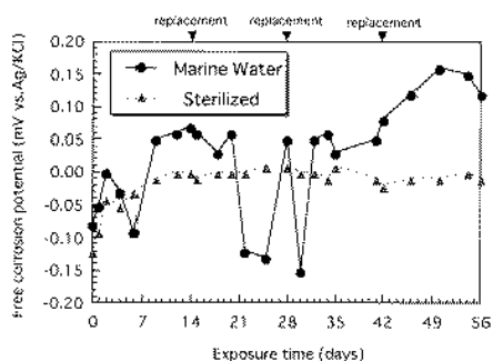
Fig.5 Variation in free corrosion potential in sterilized marine water and marine water as a function of exposure time
