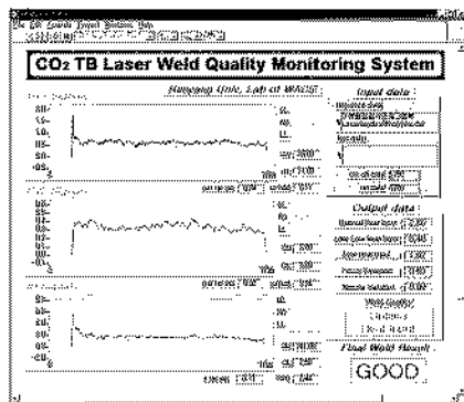
Fig. 5 Example of quality estimation program (optimal heat input)
