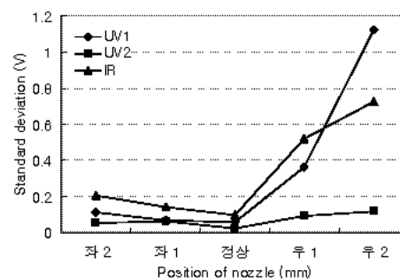
Fig. 3 Standard deviation of signals according to nozzle position
