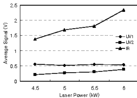
Fig. 2 Average signals according to laser power
