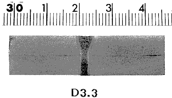
Fig. 1 Macrograph of the butt weld joint of RAEX 420MC LASER, P_L = 12\text{ kW} , v_s = 1.0\text{ m/min}
