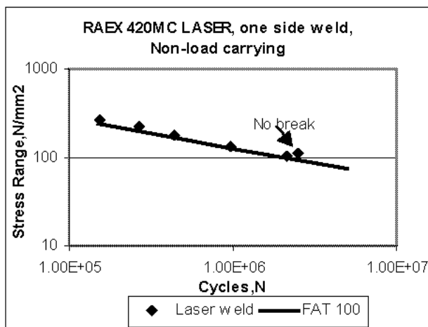
Fig. 9 Fatigue strength of the fillet weld laser-welded from one side. RAEX 420MC LASER, non-load carrying stiffener (T12/12s)
