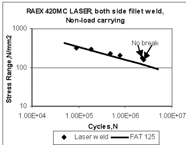
Fig. 7 Fatigue strength of the fillet weld laser-welded from both sides. RAEX 420MC LASER, non-load carrying stiffener (T12/12bs)
