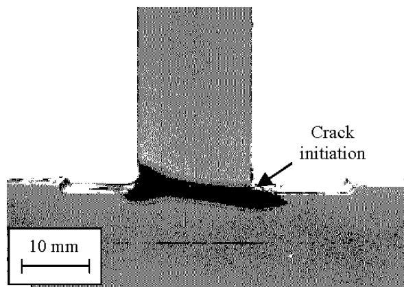
Fig. 5 Macrograph of the single side welded T-joint. RAEX 420MC LASER, P_L = 14\text{ kW} , v_s = 1.4\text{ m/min}
