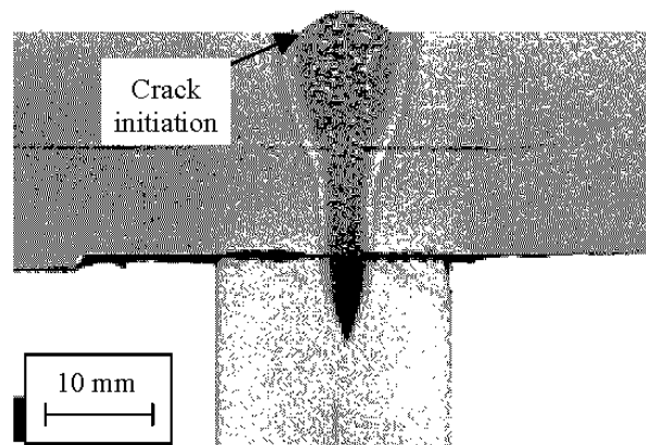
Fig. 6 Macrograph of the stake welded T-joint. RAEX 420MC LASER, P_L = 12\text{ kW} , v_s = 1.0\text{ m/min}
