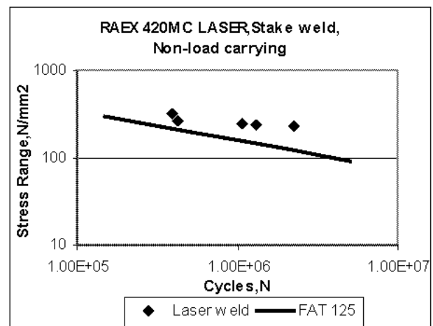
Fig. 10 Fatigue strength of the laser-welded stake weld. RAEX 420MC LASER, non-load carrying stiffener (T12/12f)
