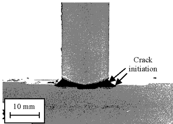
Fig. 3 Macrograph of the T-joint welded from both sides. RAEX 420MC LASER, P_L = 14\text{ kW} , v_s = 4.0\text{ m/min}
