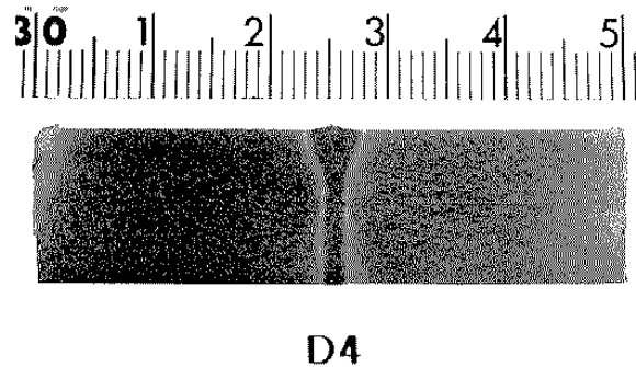
Fig. 2 Macrograph of the butt weld joint of Grade EH 36, P_L = 12\text{ kW} , v_s = 1.0\text{ m/min}
