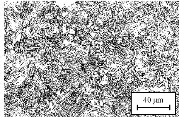
Fig. 14 Microstructure of the HAZ of Grade EH 36, P_L = 12 kW, v_s = 1.0 m/min, HV_{max} = 314
