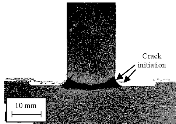
Fig. 4 Macrograph of the T-joint welded from both sides. GRADE EH 36, P_L = 7\text{ kW} , v_s = 1.12\text{ m/min}
