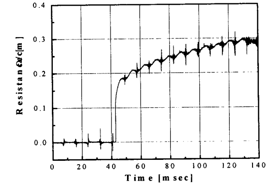
Fig. 5. Electrical properties of overall SFCL units
