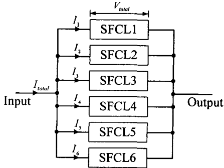
Fig. 8. Circuit diagram for increase of current ratings
