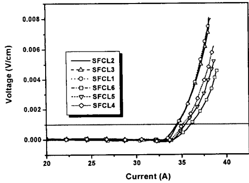
Fig. 3. I-V Curves of each SFCL elements
