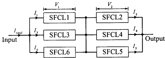
Fig. 4. Circuit diagram for increase of power ratings
