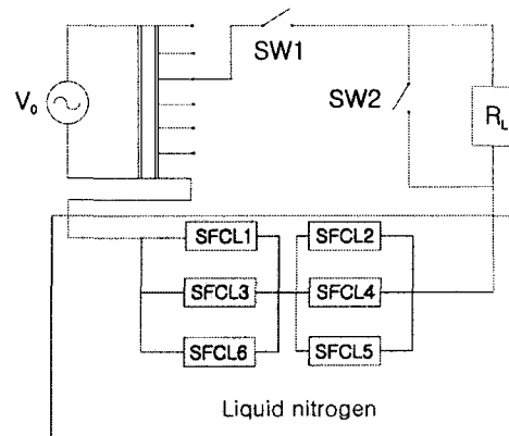
Fig. 2. Schematic setup of the test circuit
