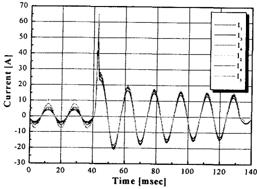
Fig. 7. Current distribution of each SFCL units
