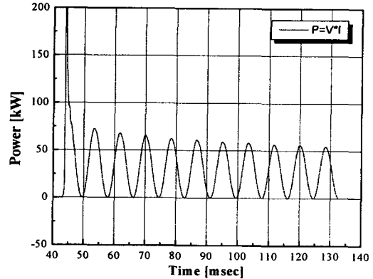
Fig. 9. Electrical properties in the parallel connection of SFCL units
