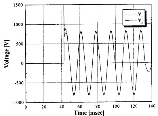
Fig. 6. Simultaneous quench properties of serially connected SFCL units
