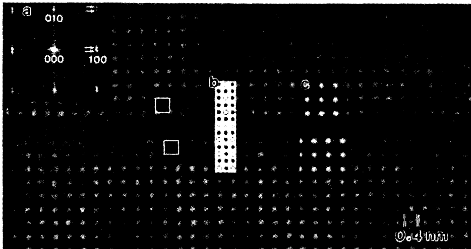
HRTEM image of \delta'/ G.P.zone multiple precipitate.
