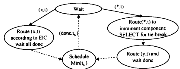
(b) Simulation Algorithm for Coordinator
