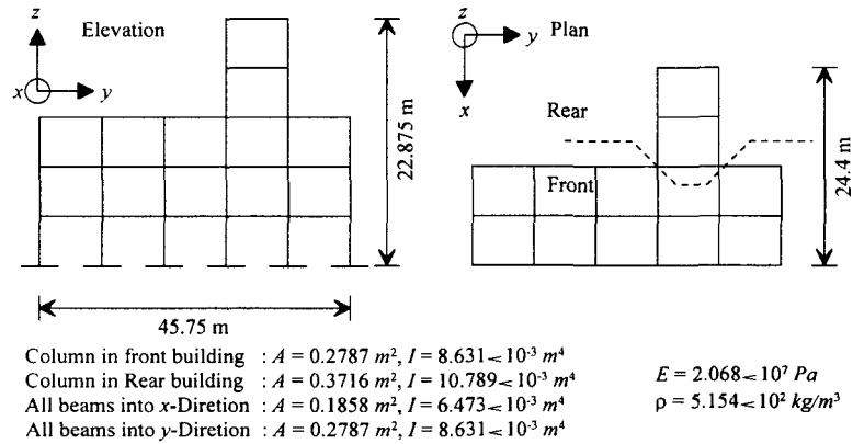
Fig. 2. Three-dimensional frame structure (DOFs: 468)
