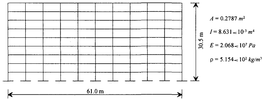
Fig. 1. Plane framed structure (DOFs: 330)
