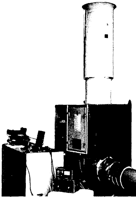
Fig. 1 Photograph of the experimental apparatus with the forced convection electric air heater tested
