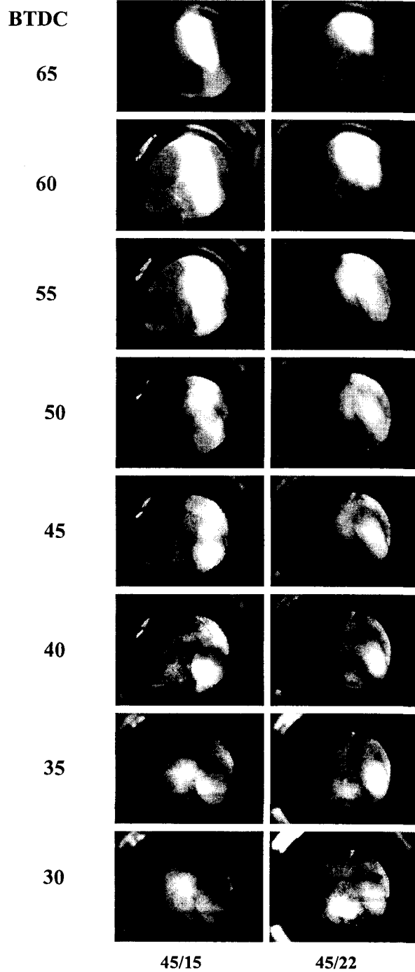
Fig.7 Ensemble averaged fuel distributions in the GDI engine with respect to injector specifications at the condition of SCV 20.
