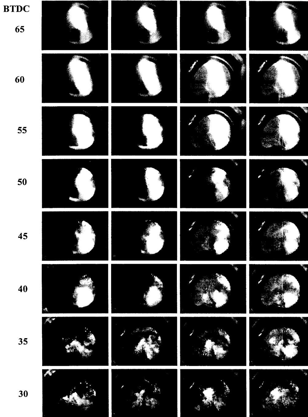
Fig.4 Fuel distributions in the GDI engine at the conditions of 45/15 injector and SCV 20.
