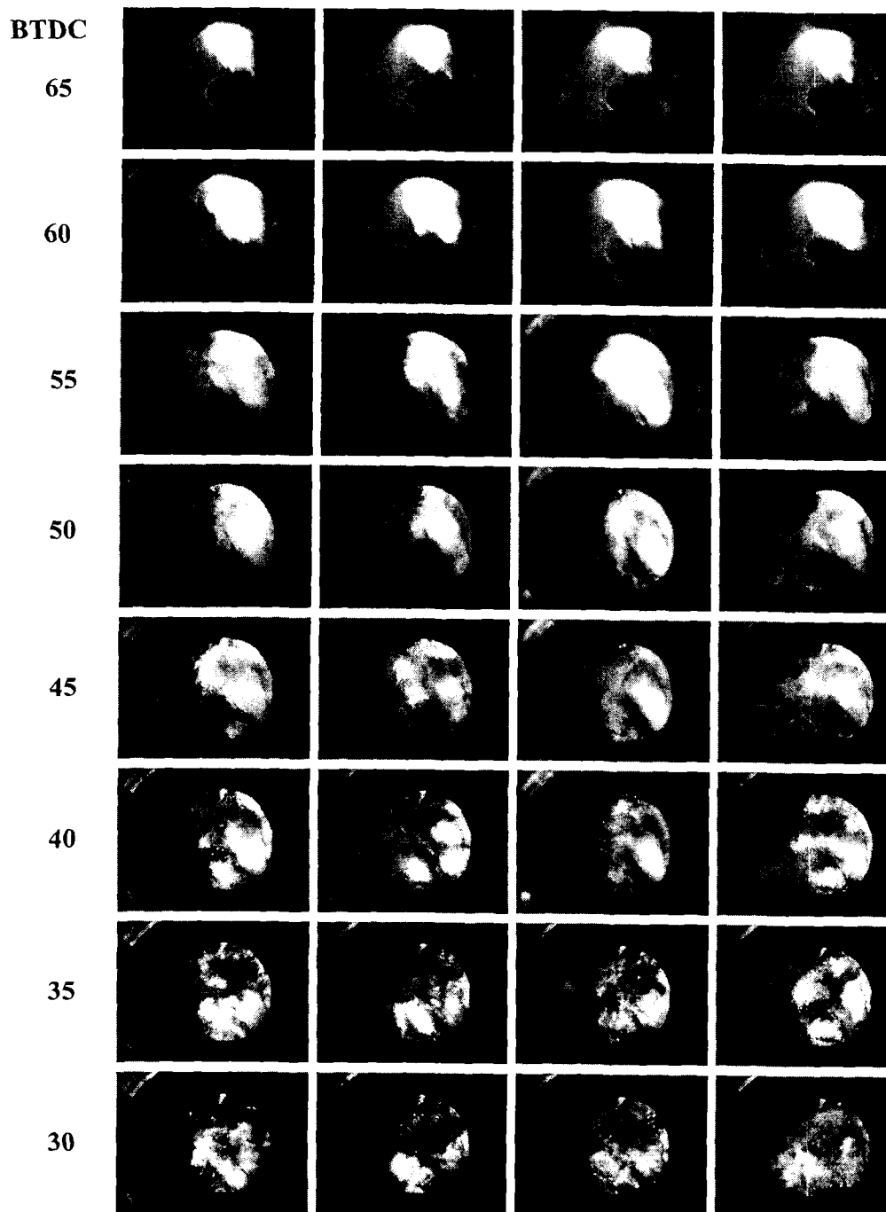
Fig.6 Fuel distributions in the GDI engine at the conditions of 45/22 injector and SCV 20.
