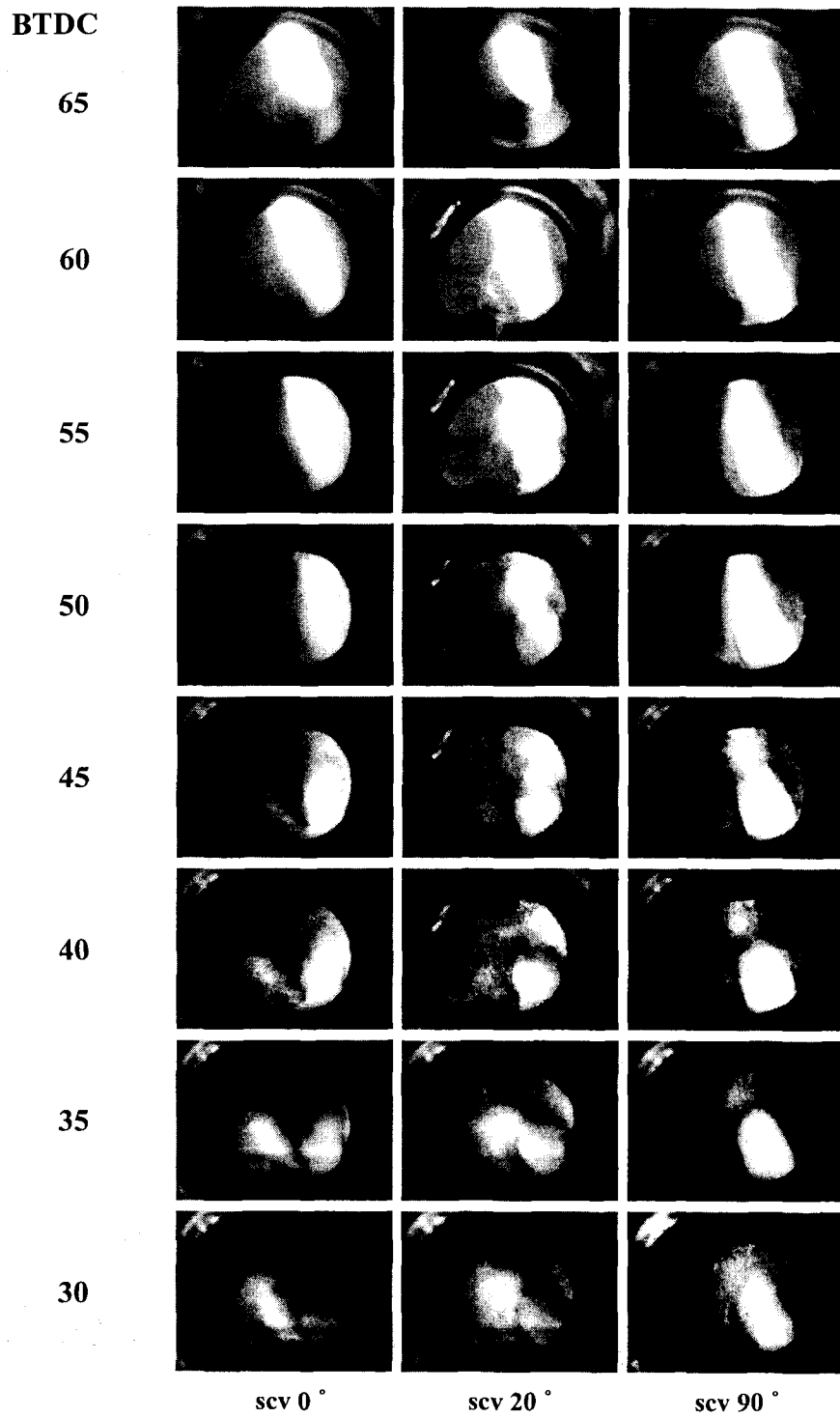
— Fig.5. Ensemble averaged fuel distributions in the GDI engine with respect to SCV opening
