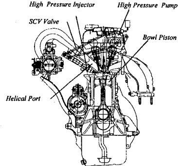
Fig.1 Layout of the GDI engine
