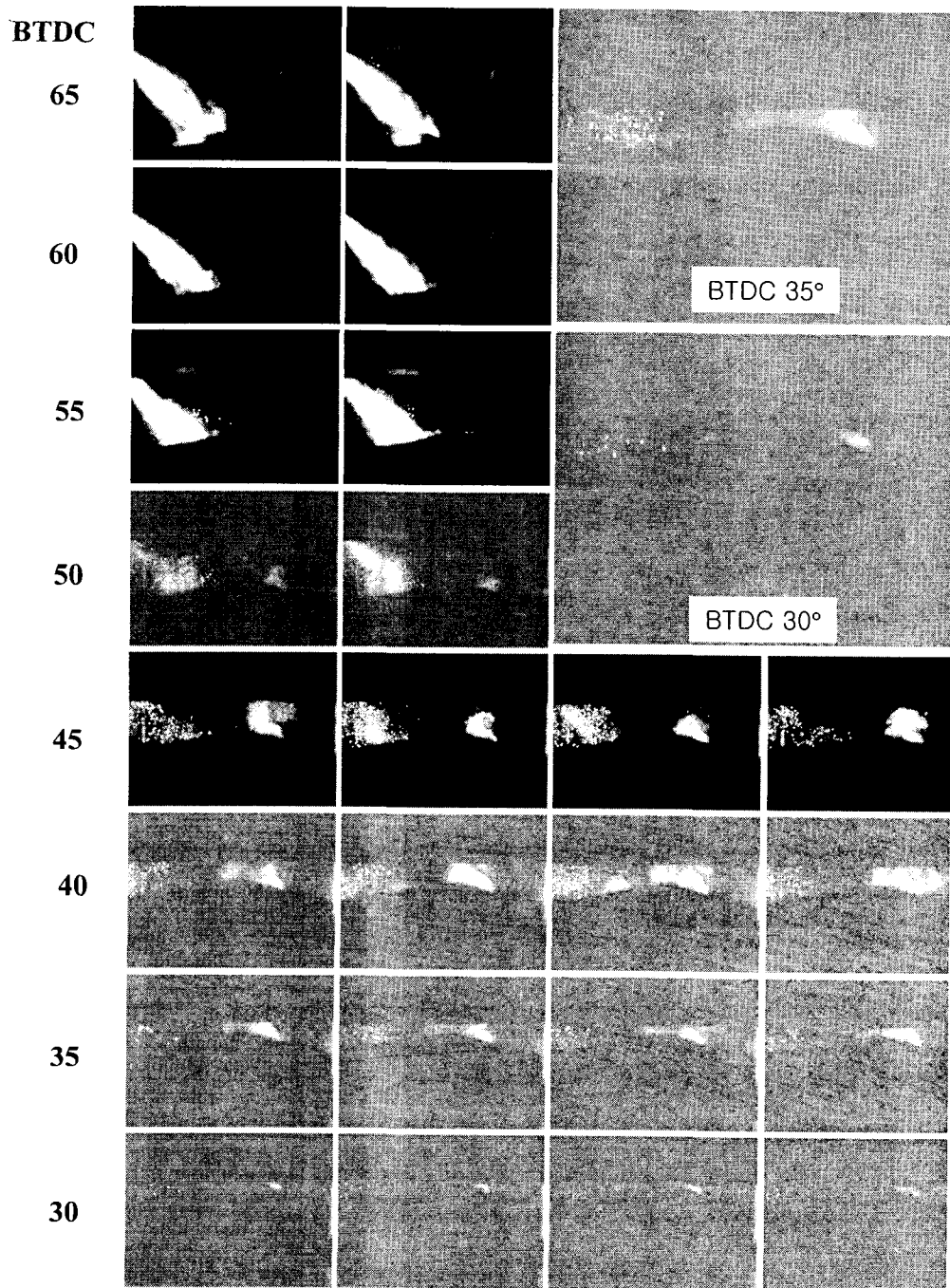
Fig.3 Fuel distributions in the GDI engine at the conditions of 45/15 injector and SCV 20.
