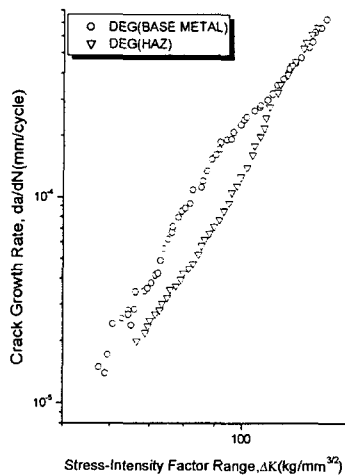
Fig. 8 \Delta K-da/dN diagram of HAZ and base metal for degraded material
