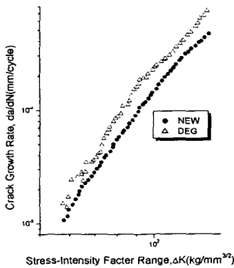
Fig. 5 \Delta K-da/dN diagram of new material and degraded material for base metal
