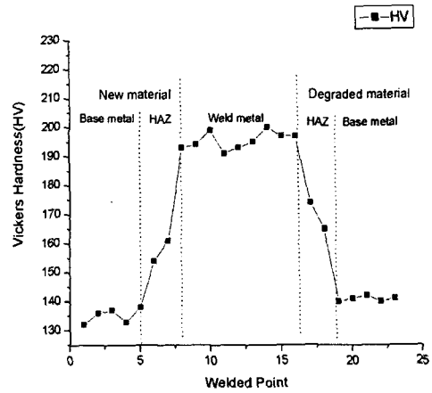
Fig. 2 Diagram of Vickers hardness value by welded position
