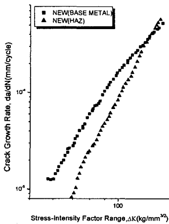
Fig. 7 \Delta K-da/dN diagram of HAZ and base metal for new material
