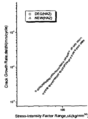
Fig. 6 \Delta K-da/dN diagram of new material and degraded material for HAZ
