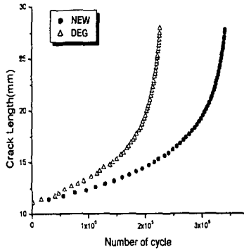
Fig. 3 Crack length-cycle of base metal
