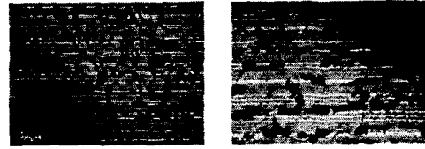
(a) New material (b) Degraded material Fig. 1 Micro-structure of base metal
