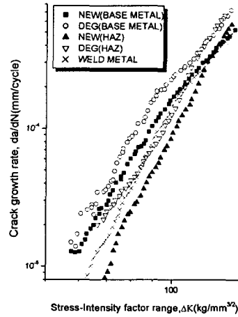
Fig. 9 \Delta K-da/dN diagram of HAZ, base metal and weld metal for degraded material and new material
