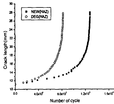
Fig. 4 Crack length-cycle of HAZ
