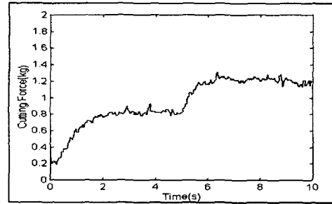
Fig. 2.9 Average Cutting Force Signal due to Step Change in Feed under Constant Spindle Speed
