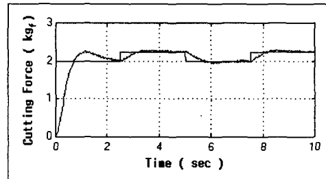
Fig. 4.5. Cutting Force Control under Two Degree-of Freedom Controller with Modelling Error
