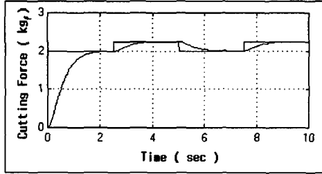
Fig. 4.1. Cutting Force in Reference Model
