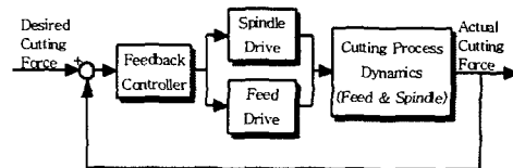
Fig. 3.1 Control System Structure for Simultaneous Control of Spindle Speed and Feed Speed
