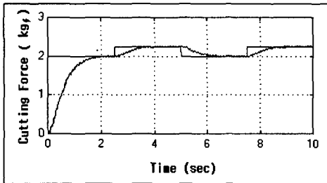
Fig. 4.2. Cutting Force Control under Two Degree-of Freedom Controller
