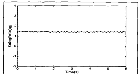
Fig. 2.3 Averaged Cutting Force Signal in Milling Process
