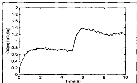
Fig. 2.5 Average Cutting Force Signal due to Step Change in Spindle Speed Under Constant Feed Speed
