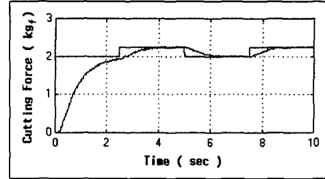
Fig. 4.4. Cutting Force Control under Two Degree-of Freedom Controller with Step Disturbance
