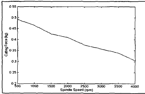
Fig. 2.6 Spindle Speed versus Cutting Force under 0.01m/s Feed
