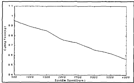
Fig. 2.7 Spindle Speed versus Cutting Force under 0.02m/s Feed
