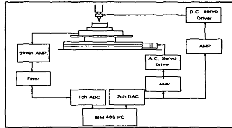
Fig. 2.1 Schematic Diagram for Data Acquisition and Control
