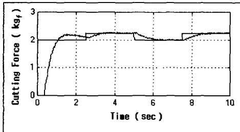
Fig. 4.3. Cutting Force Control under Two Degree-of Freedom Controller with Impulse Disturbance
