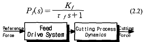
Fig. 2.8 Block Diagram with Constant Spindle Speed
