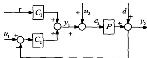
Fig.3.2 Two Degree-of-Freedom Control System
