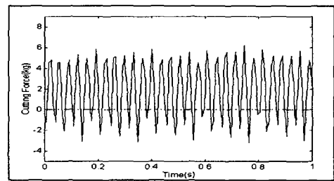
Fig. 2.2 Raw Cutting Force Signal in Milling
