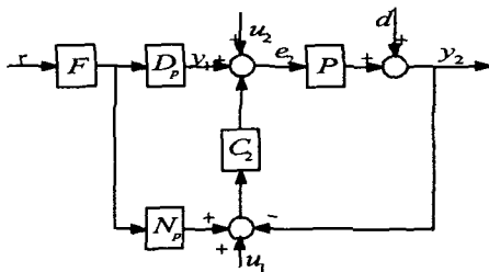
Fig.3.3 Modified Two Degree-of-Freedom Control System
