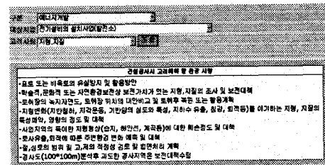
Fig 10. Environment influence
