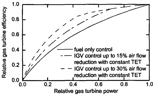
Fig. 8 Effect of power control scheme on part load efficiency of a regenerative gas turbine.
