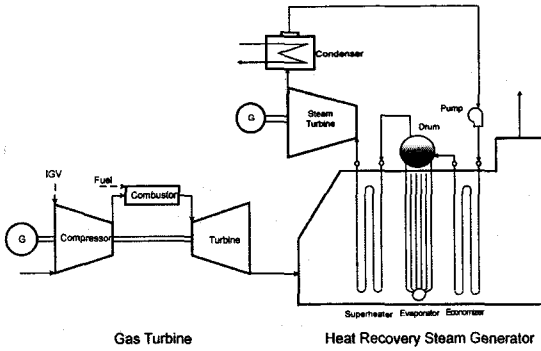
Fig. 2 Schematic diagram of the combined cycle power plant adopting a single-pressure bottoming system.
