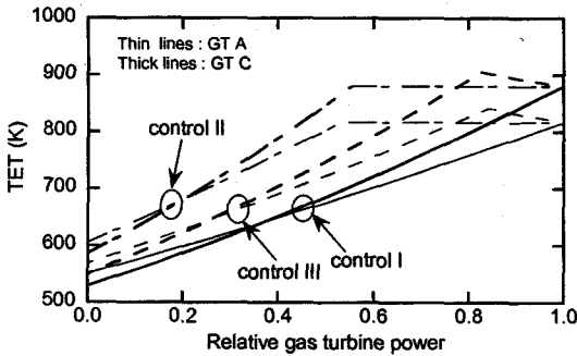
Fig. 4 Variation in turbine exhaust temperature.
