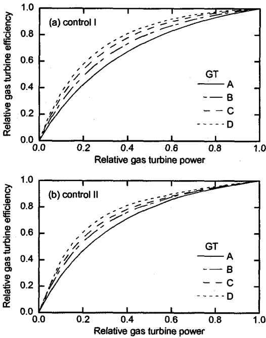
Fig. 3 Variation in gas turbine efficiency during part load operation.
