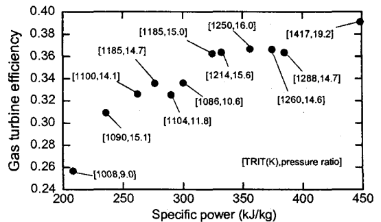
Fig. 1 Design performance data for commercial gas turbines for electric power generation. (1)
