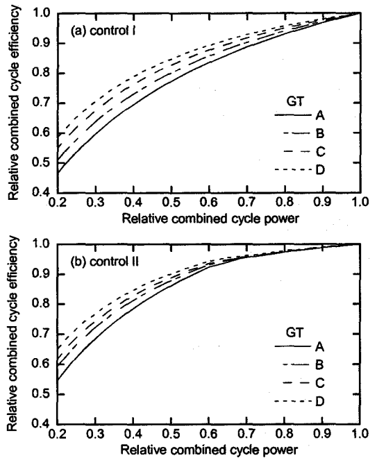
Fig. 6 Variation in combined cycle efficiency during part load operation.
