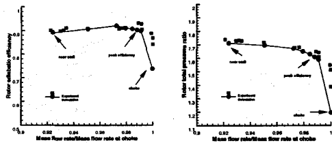
Fig. 3 NASA Rotor67 performance at design speed
