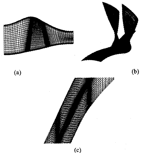
Fig. 2 Computational grid for NASA Rotor67; (a) Meridional plane (b) Blade surfaces and hub wall (c) Tip clearance region
