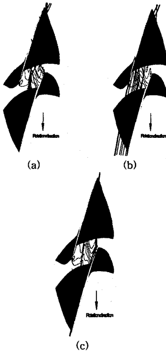
Fig. 7 Particle traces at peak efficiency operating point; (a)coming from the tip clearance, (b)coming from upstream, (c)coming from upstream close to blade surface
