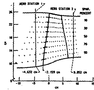
Fig. 1 Meridional view of Rotor67 showing measurement locations
