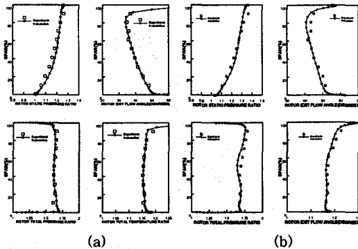
Fig. 4 Predicted and measured exit survey data (a) peak efficiency operating point (b) near stall operating point
