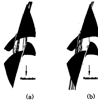
Fig. 8 Particle traces near stall operating point; (a) coming from tip clearance,(b)coming from upstream
