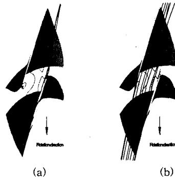
Fig. 6 Particle traces at choke operating point; (a)coming from the tip clearance, (b)coming from upstream
