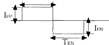
Fig. 5 Schematic of EN ratio
