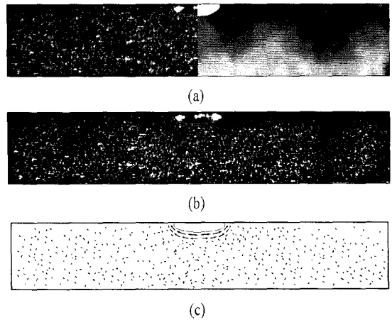
Fig.7 No flow Region (a) (b) : explain same as Fig.6 (c) Redrawing Flow pattern from the Image (b)
