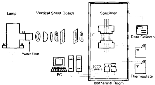
Fig. 1 Experimental setup for temperature and flow field visualization
