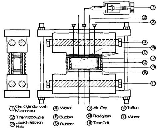
Fig. 2 Schematic of Exp. Specimen
