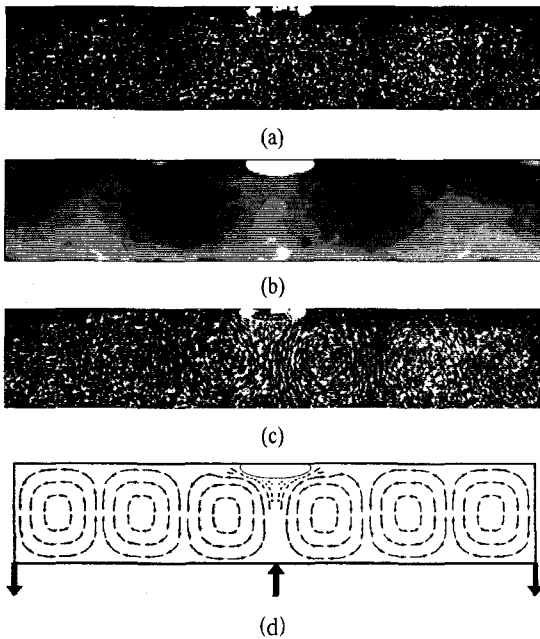
Fig.9 Steady State for the Reversed state (a) (b) (c) : explain same as Fig.6 (d) Redrawing flow pattern from the Image(c)
