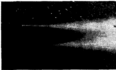
Fig. 1 Conical Steam Jet (Nozzle ID : 20 mm, Steam Mass Flux : 280 kg/m 2 -s, Pool Temp. : 40 °C)
