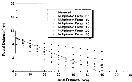
Fig. 6 Steam Jet Cavity with the Change of Multiplication Factor (Nozzle ID : 20 mm, case 1)
