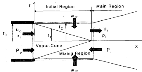
Fig. 3 Control Volume for a Conical Steam Jet
