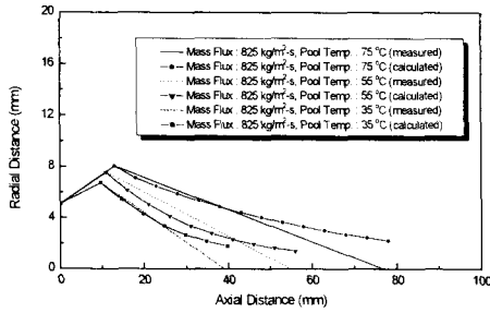
Fig. 8 Steam Jet Cavity with the Change of Pool Temp. (Nozzle ID : 10.15 mm)
