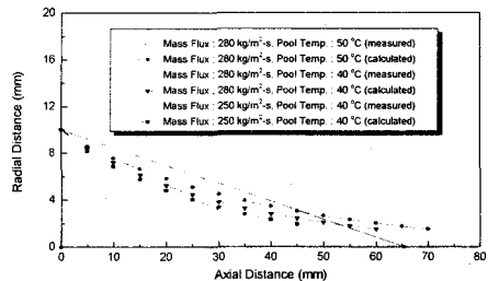
Fig. 7 Steam Jet Cavity with the Change of Steam Mass Flux and Pool Temp. (Nozzle ID : 20 mm)
