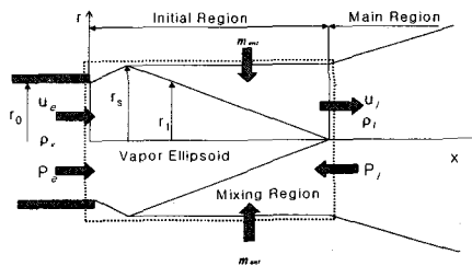
Fig. 4 Control Volume for an Ellipsoidal Steam Jet
