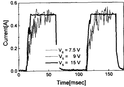
Figure 5. Control Current to Step Control Voltage in Load 2
