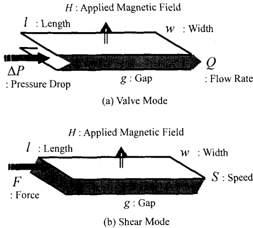
Figure 6. Basic Operational Modes [Carlson et al., 1995]
