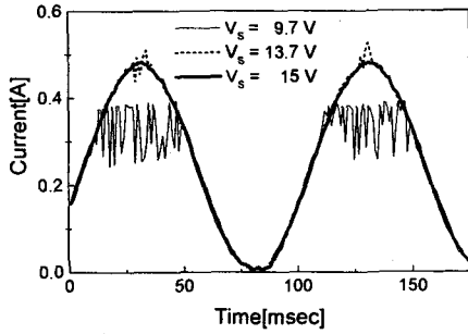
Figure 2. Control Current to Sinusoidal Control Voltage in Load 1
