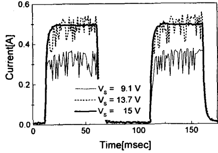
Figure 4. Control Current to Step Control Voltage in Load 1
