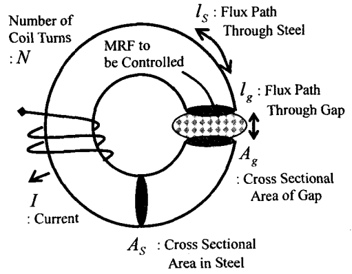
Figure 7. Magnetic Circuit of MRF Device [Weiss et al., 1993]
