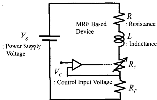
Figure 8. Electric Circuit of MRF Device with Current Amplifier [Maslen et al., 1989]
