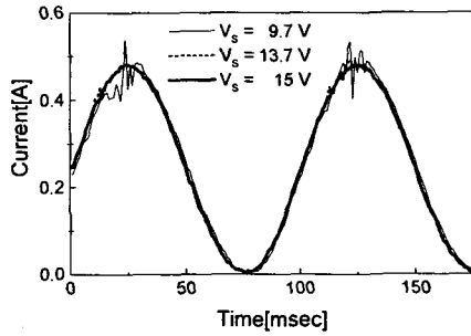
Figure 3. Control Current to Sinusoidal Control Voltage in Load 2
