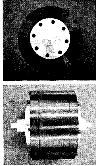
Figure 1. Rotary MR Damper for Electronically Controlled Power Steering [Jung and Park, 1998 and 1999]
