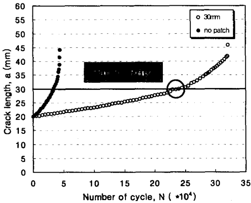
Fig. 8 Crack length versus fatigue cycle for 30mm patch configuration
