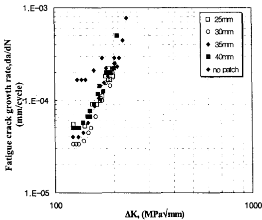
Fig. 12 Crack growth ratio versus \Delta K diagram for the various patch length
