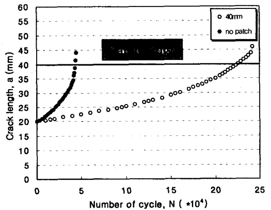
Fig. 10 Crack length versus fatigue cycle for 40mm patch configuration
