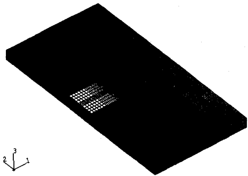
Fig. 3 FEM model of single sided repair
