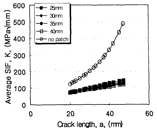
Fig. 6 Average SIF versus crack length for patch configurations
