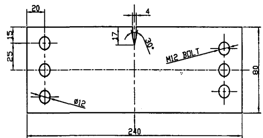
Fig. 1 Configuration of test specimen (unit : mm)
