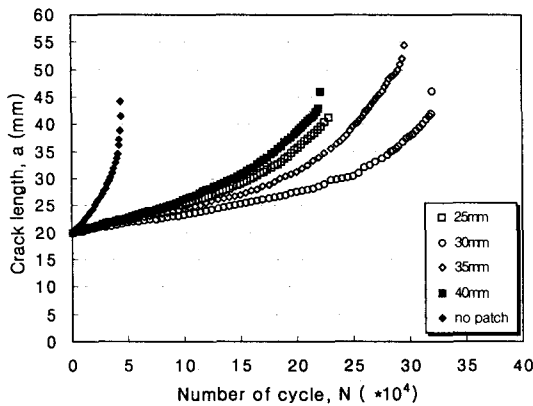
Fig. 11 Crack length versus fatigue cycle at the various patch length
