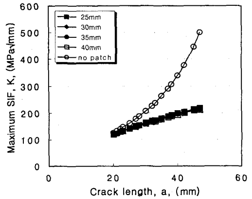
Fig. 4 Maximum SIF versus crack length for patch configurations
