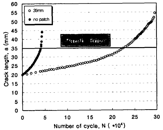
Fig. 9 Crack length versus fatigue cycle for 35mm patch configuration
