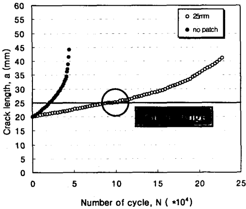
Fig. 7 Crack length versus fatigue cycle for 25mm patch configuration
