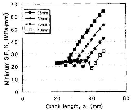
Fig. 5 Minimum SIF versus crack length for patch configurations
