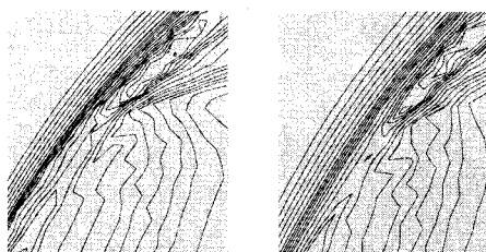
(a) Density for Mach 5.11 (b) Density for Mach 6.46 around the reaction front
