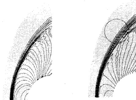
(a) Temperature (b) Density
