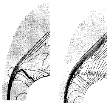
(b) Temperature (c) Density
