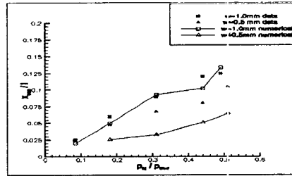
Fig. 10 Separation length of slot total pressure ratio
