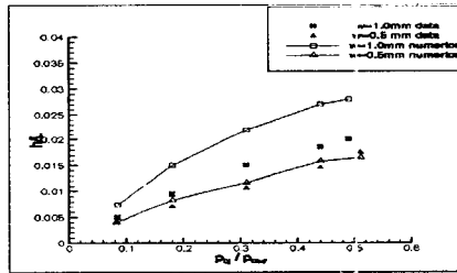
Fig. 11 Height of mach surface of slot total pressure ratio
