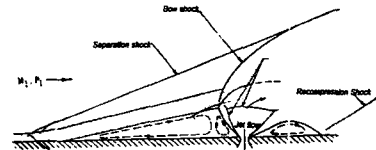
Fig. 1 Slot injection geometry
