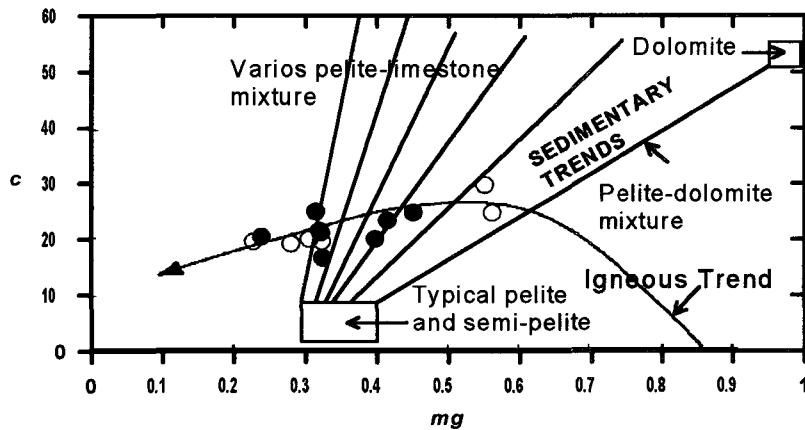
Fig. 1. Niggli mg-c plot ( mg=Mg/(Ca+Mg+total\ Fe+Al) , c=(Ca \times 100)/(Mg+Mn+total\ Fe) slightly modified after Leake(1964) for Pyeonghae(open circles) and Wonnam(solid circles) amphibolites.
