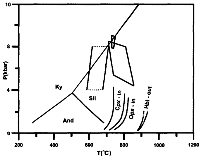
Fig. 3. P-T conditions of study area. Filled area is Pyeonghae Formation and open area is Wonnam Formation.
