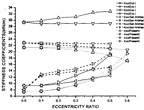
Fig. 3 Comparison of stiffness coefficients between experimental(—) and predictions(San Andres(---) ; present analysis(····)).
