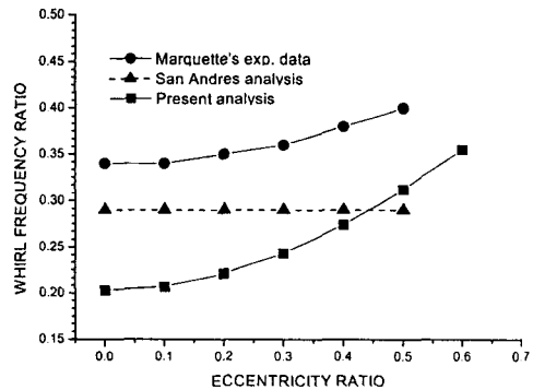
Fig. 7 Comparison of whirl frequency ratio between experimental(circle) and predictions(San Andres(triangle) ; present analysis(square)).
