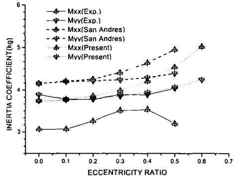
Fig. 6 Comparison of added mass coefficients between experimental(—) and predictions(San Andres(---) ; present analysis(···)).
