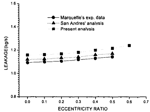
Fig. 2 Comparison of leakage between experimental(circle) and predictions(San Andres(triangle) ; present analysis(square)).
