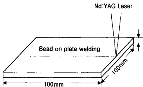
Fig. 1 Dimension of specimen
