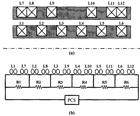
Fig.2. (a)Actively shielded MRI (b)Quench protection circuit for act shielded MRI coil
