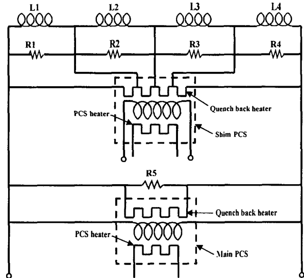
Fig.4. Quench protection circuit for shim
