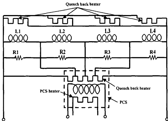
Fig.3. Fast quench protection coil by h back heater
