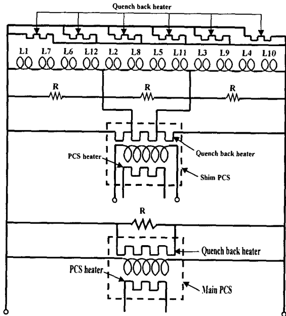
Fig.5. Suggested quench protection circ
