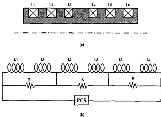
Fig.1. (a)Six section main coil (b)Qu protection circuit for the maintenanc symmetric field
