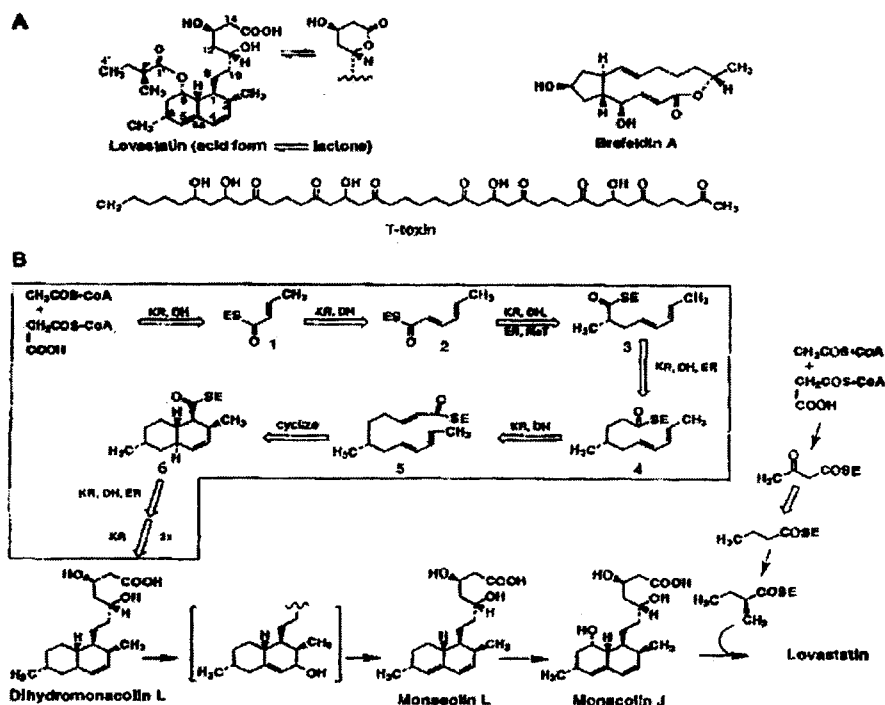
Fig. 1. (A) Typical reduced fungal polyketides. (B) Lovastatin biosynthetic hypothesis. The boxed region shows the set and order of reactions thought to be necessary for the biosynthesis of dihydromonacolin L, the first recognized intermediate in lovastatin biosynthesis.
