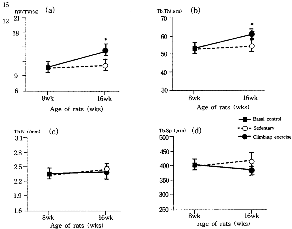
Fig. 4. Structural indices of the proximal tibial metaphysis in climbing exercise rats. (a) Bone volume(BV/TV, %), (b) trabecular thickness(Tb.Th, \mu\text{m} ), (c) trabecular number (Tb.N, /mm), (d) trabecular separation (Tb.Sp, \mu\text{m} ). Values are mean \pm SEM.
